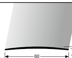
167 U ungebohrt undrilled non percé
