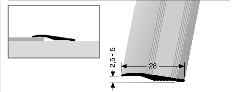
264 U ungebohrt undrilled non percé
