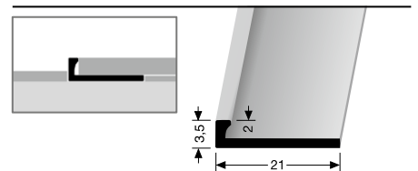
299 U ungebohrt undrilled non percé
