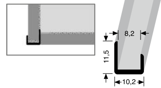
178 U \hat{=} 8,2 mm ungebohrt undrilled non percé
