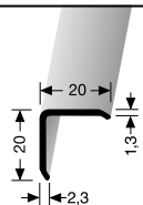
271 U ungebohrt undrilled non percé
