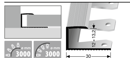
213 EB ⇄ 12 - 13,2 mm offen gestanz open punched estampé ouvert
