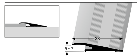
265 U ungebohrt undrilled non percé
