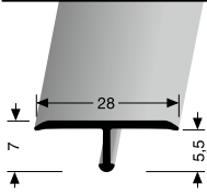
293 U ungebohrt undrilled non percé
