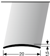
472 U ungebohrt undrilled non percé
