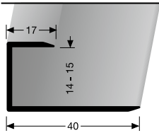
204 U ungebohrt undrilled non percé
