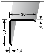
273 U ungebohrt undrilled non percé
