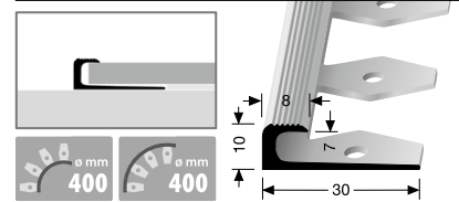
805 EB ⇄ 7 mm offen gestanz open punched estampé ouvert
