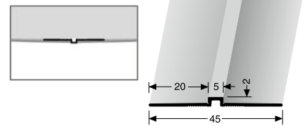
170 U ungebohrt undrilled non percé
