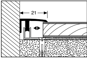
557 H \updownarrow 7 – 12 mm
