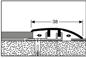
576 XL \updownarrow 3,5–6,5 mm (4–11 mm*)
