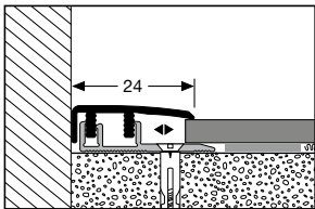
577 XL \updownarrow 3,5–6,5 mm (4–11 mm*)
