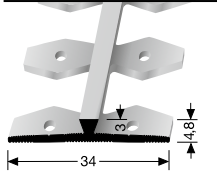
365 EB ⇄ 3 mm
