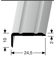
236 U/FW-L ungebohrt undrilled non percé
