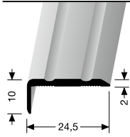
236 U/FW ungebohrt undrilled non percé
