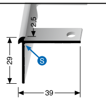
870 EB ± 2,5 mm
