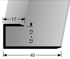
202 U ungebohrt undrilled non percé
