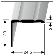
235 U/FW-L ungebohrt undrilled non percé
