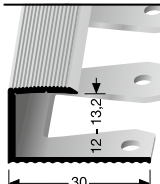
213 EB ⇄ 12–13,2 mm
