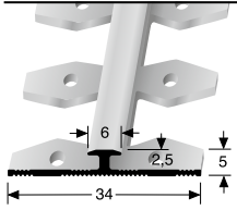
363 EB ⇄ 2,5 mm
