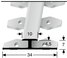
368 EB ⇄ 4,5 mm
