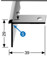
871 EB \updownarrow 3 mm
