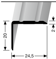
235 U/FW-R ungebohrt undrilled non percé
