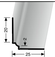
160 U ungebohrt undrilled non percé
