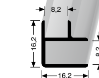
164 U ± 8,2 mm ungebohrt undrilled non percé
