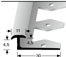
345 EB ⇄ 4,5 mm
