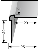
150 U ungebohrt undrilled non percé
