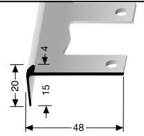
861 EB ± 4 mm
