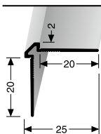
155 U ungebohrt undrilled non percé
