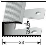
210 EB ⇄ 7,2–8,2 mm
