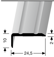
236 U/FW-R ungebohrt undrilled non percé
