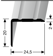
235 U/FW ungebohrt undrilled non percé
