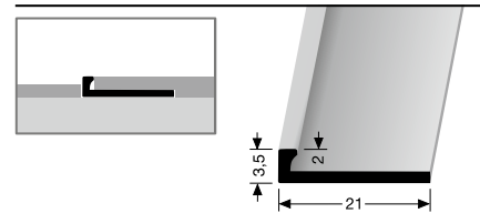
299 U ungestanz unpunched non estampé
