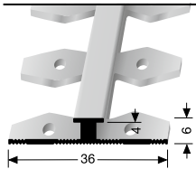
366 EB ⇄ 4 mm
